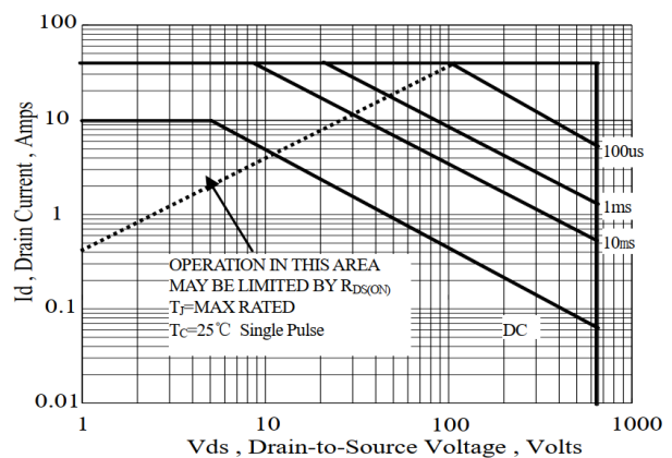
Fig 12 Safe Operation Area (ITO-220AB)
