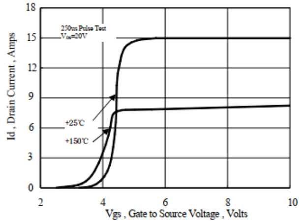
Fig 8 Transfer Characteristics
