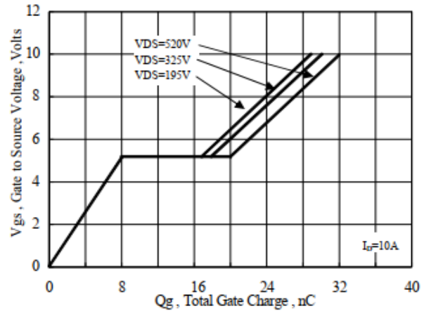
Fig 10 Gate-Charge Characteristics
