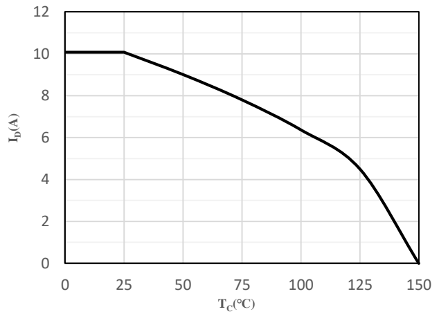
Fig 2 Drain Current
